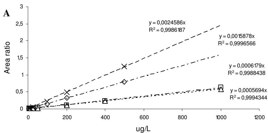
Figure 1. Lineary of calibration curve of methylated (A) and ethylated (B) compounds.
